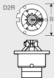
P32d-3 IEC 7004-111
