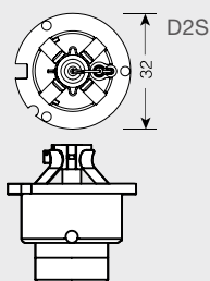
P32d-2 IEC 7004-111
