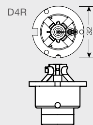
P32d-6 IEC 7004-111
