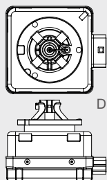
PK32d-2 IEC 7004-111
