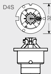
P32d-5 IEC 7004-111
